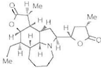
Tuberostemonin
