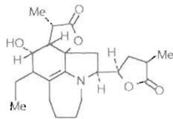
Oxotuberostemonin
